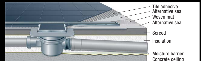
Thin mortar bed seal using channel flange
