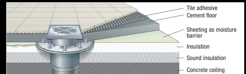
Seal through sealing sheet and pressure sealing flange
