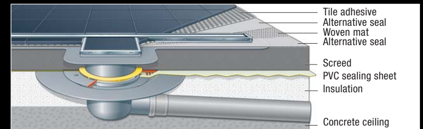
Conventional seal using sheeting
