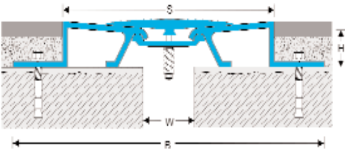
747-A01-050 Floor/Floor
