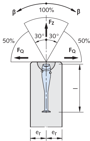
Load capacity and reinforcement of Spherical Head Tilt-up Anchor
