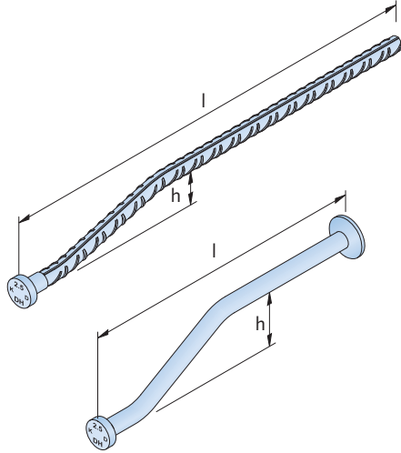
Dimensions of Spherical Head Anchor, offset versions
