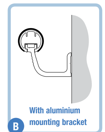
Tubular handrail MCE 40/45
