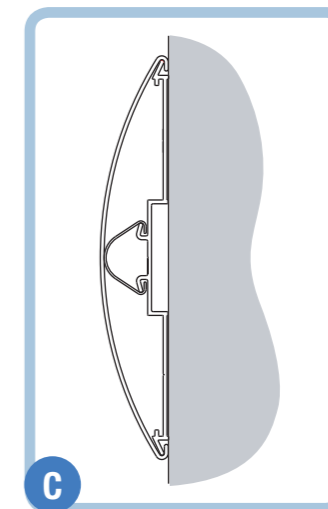
Crash rail SCR 80M
