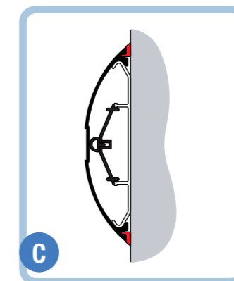
Smooth Crash rail Aronde 170 Duo
