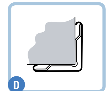
Surface Mounted Corner guard SSM 20 C/S Acrovyn® Faux Brushed Silver
