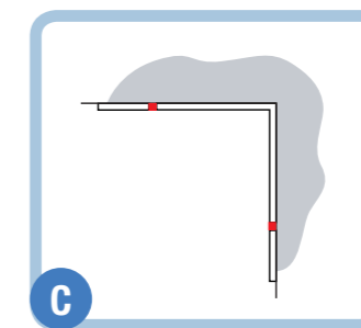
C/S Acrovyn® sheet Thermoformed internal angle 90° with welded joint to the adjacent sheet
