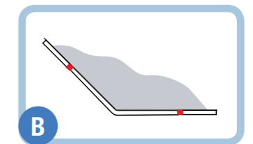
C/S Acrovyn® sheet Thermoformed external angle 135° with welded joint to the adjacent sheet
