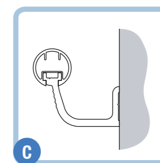
Tubular handrail Vision
