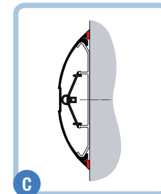
Smooth Crash rail Aronde 170
