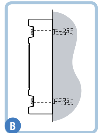
C/S Stelatex® Rubber Bumper guard 200 W 50
