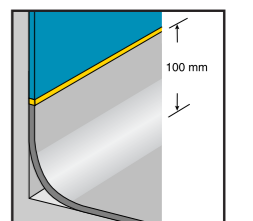
Heat-sealed junction with flexible flooring
