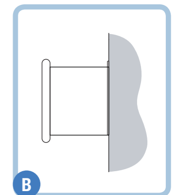
Full aluminium Bumper handrail ECR 32 A
