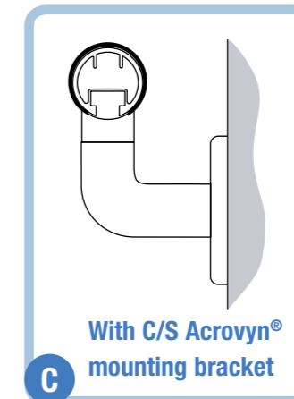
Tubular handrail MCE 40/45
